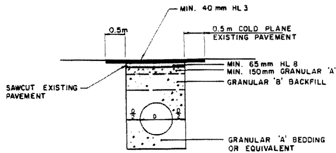
TRENCH RESTORATION
