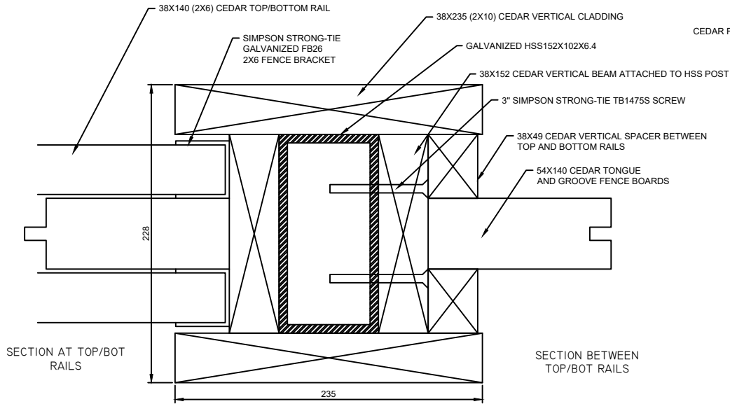
POST SECTION SCALE 1:2
