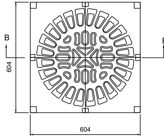
GRATE PLAN
