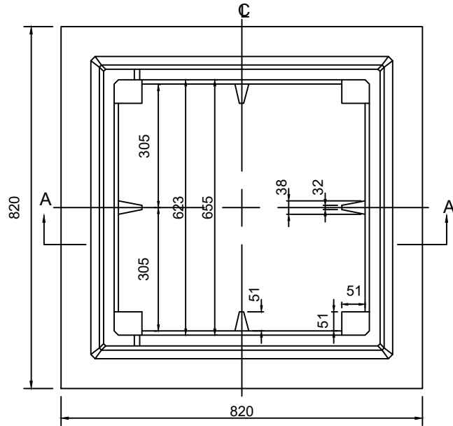
FRAME PLAN
