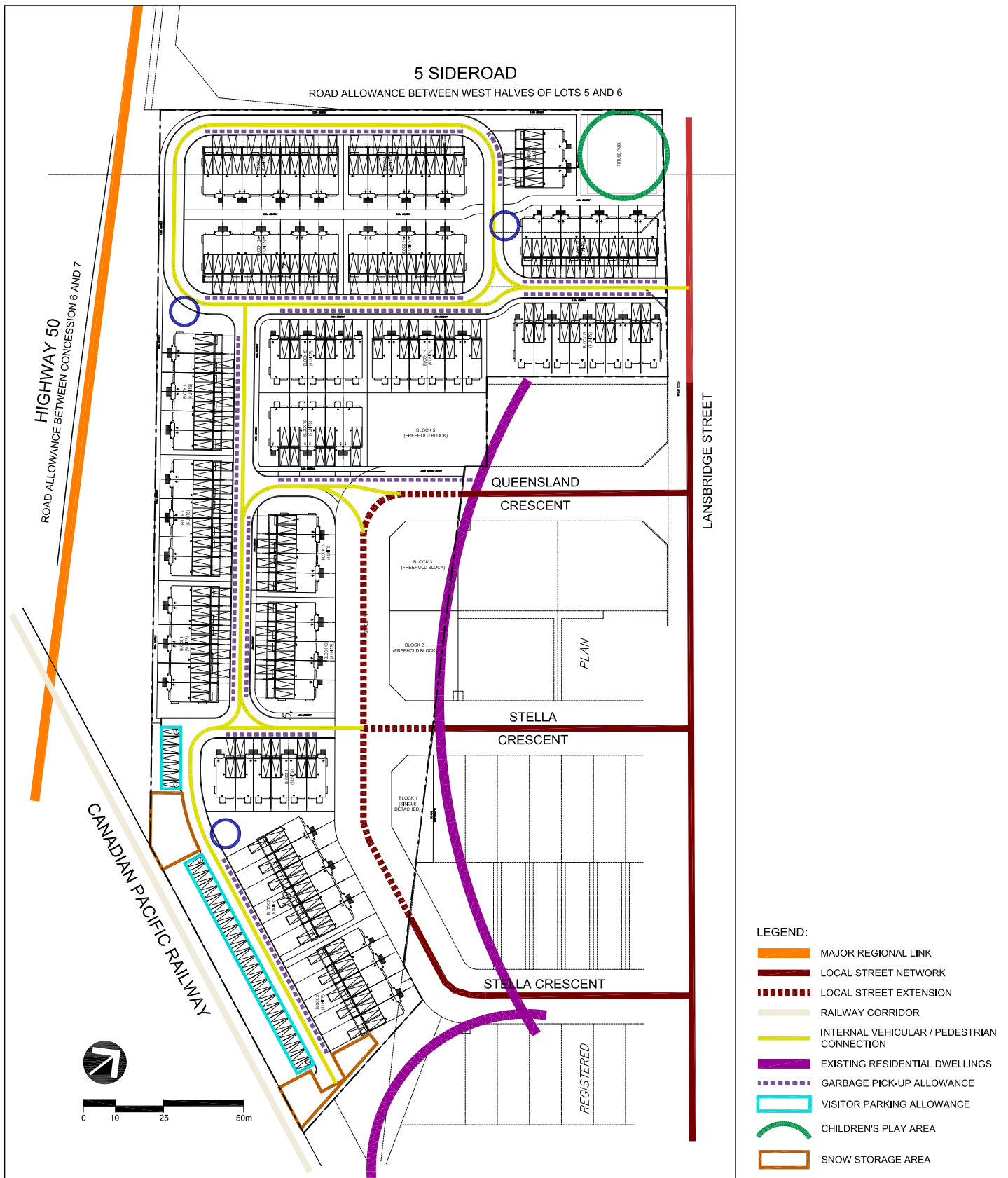
Figure 2.1 - Conceptual Opportunities and Constraints Plan
