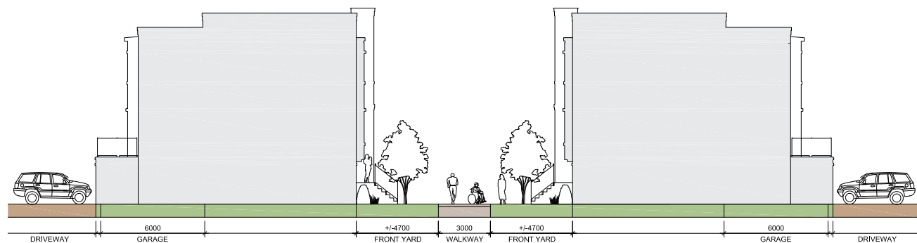
Figure 3.1.2a - Conceptual section of typical townhouse and courtyard / walkway interface.
