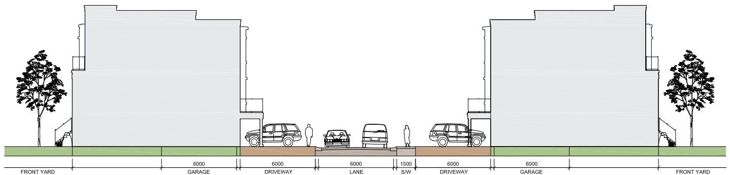
Figure 3.1 - Conceptual section of typical townhouse and lane interface.
