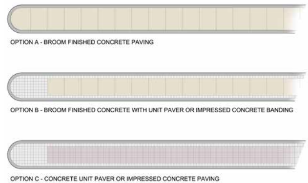
Figure 6.4c – Conceptual 2.0m wide island median paving options. To enhance the streetscape character, decorative paving shall be considered as an alternative to broom finished concrete.
