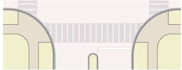
Figure 6.10.7a– Crosswalk Option A, zebra striped
