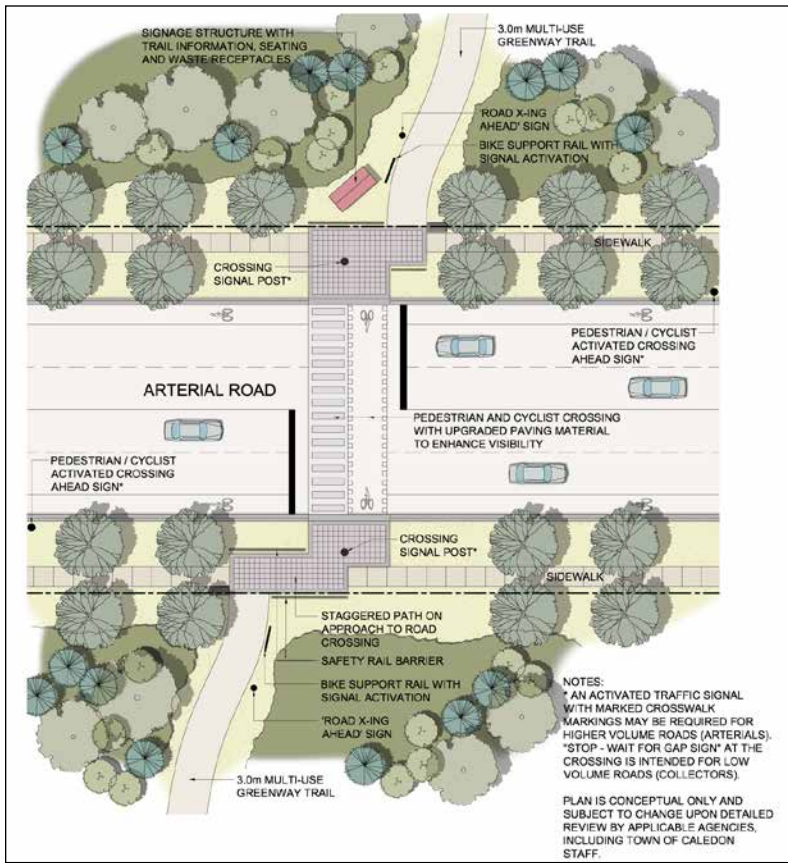
Figure 5.4h – Conceptual plan option for a potential mid-block trail crossing at a higher volume (arterial) road. The crossing will be pedestrian/cyclist activated, whether fully signalized or as an activated crosswalk with amber light sequence.
