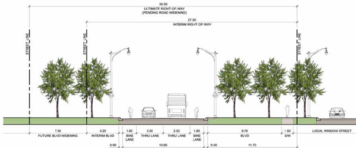
Figure 6.5c – Conceptual treatment along Chinguacousy Road between Mayfield Road and the north limit (27.5m interim ROW / 35.0m ultimate ROW) with 2 thru lanes, on-street bike lanes and street trees in grass boulevard on both sides (looking north). The right-of-way width allows for future expansion of the roadway to 4 lanes.
