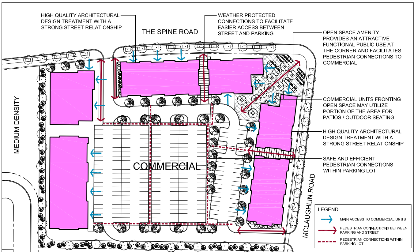
Figure 8.6.1j – Conceptual demonstration plan illustrating the key principles for siting buildings within a commercial block, particularly within the Urban Village Centre, with a strong building-street relationship and where a balance of direct street access and rear parking lot access to individual units is achieved.
