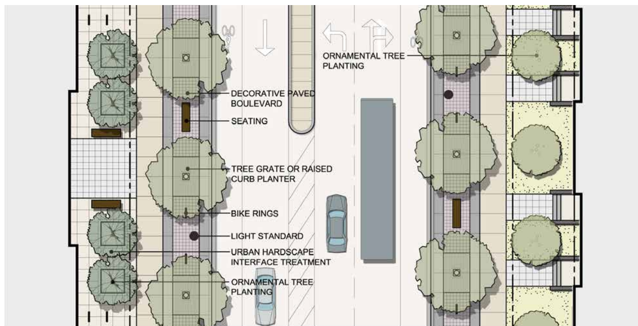
Figure 6.4.2b – Section B2-B2: Conceptual Spine Road treatment east of McLaughlin Road (toward intersection) (29.0m ROW) with 2 thru lanes, left turn lane, island median, on-street bike lanes and street trees in grates adjacent the Community Park/ Recreation Centre and high-density residential (looking west).
