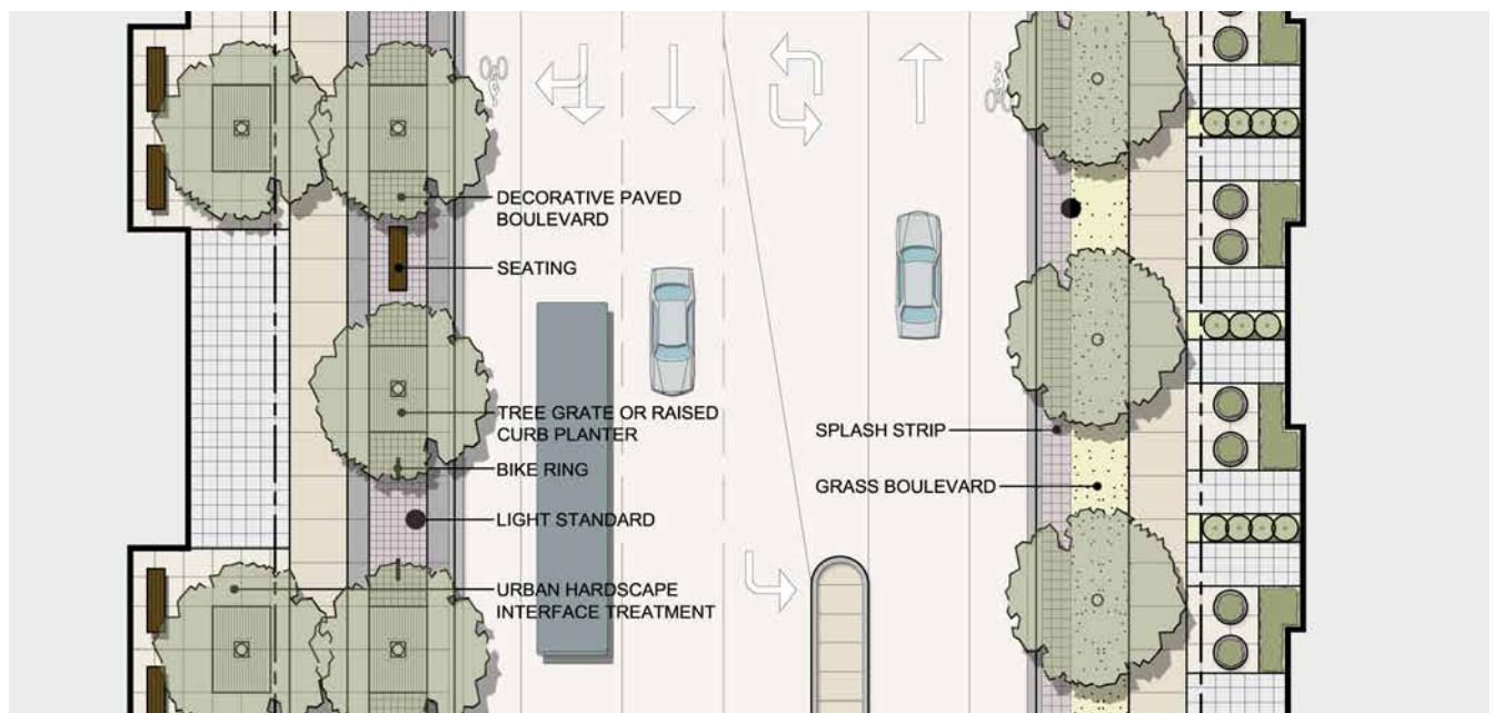
Figure 6.4.2e – Section B3-B3: Conceptual Spine Road treatment west of secondary school entrance (32.0m ROW) with 2 thru lanes, right turn into school or thru, left turn lane, island median, on-street bike lanes and street trees in grass boulevard (adjacent to medium density) or hard surface treatment (adjacent to school) (looking west).
