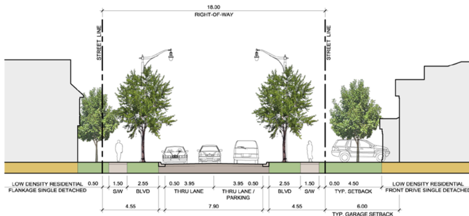
Figure 6.7 – Conceptual typical treatment for Local Roads with 2 thru lanes, sidewalks on both sides, parking on one side and street trees in grass boulevard.
