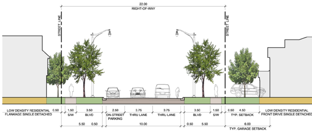
Figure 6.6c – Conceptual typical treatment for Collector Roads A, B, C, D, E, F and G (22.0m ROW) with 2 thru lanes, on-street parking on one side and street trees in grass boulevard.
