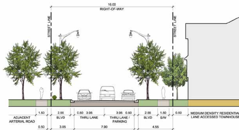
Figure 6.8 – Conceptual typical treatment for Window Streets with 2 thru lanes, parking on one side and street trees in grass boulevard.
