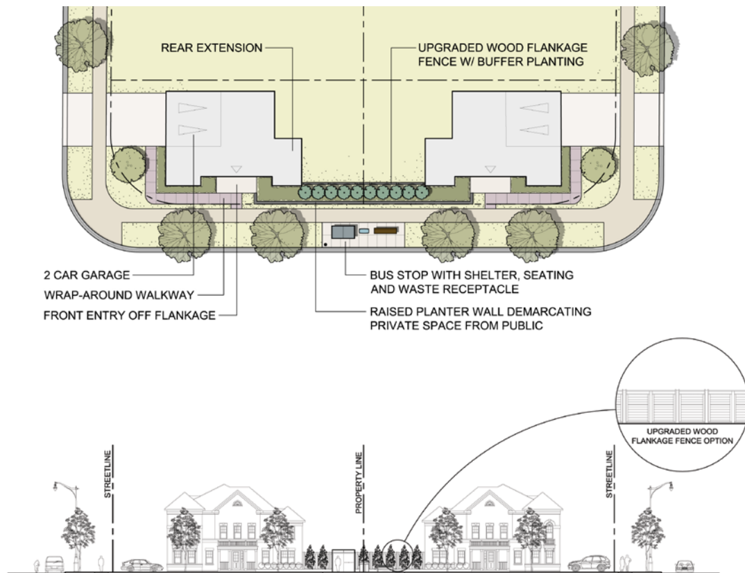
Figure 6.10.2e – Conceptual flankage treatment depicting built form with rear yard extension conventional, wrap-around walkway and upgraded wood flankage fence. The flankage treatment provides an attractive backdrop for a mid-block bus stop.
