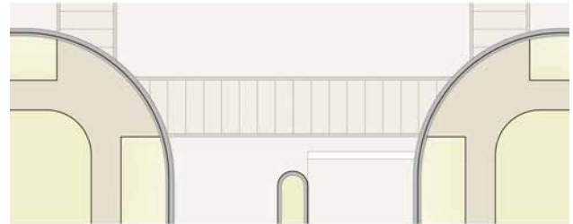
Figure 6.10.7b– Crosswalk Option B, broom finished concrete
