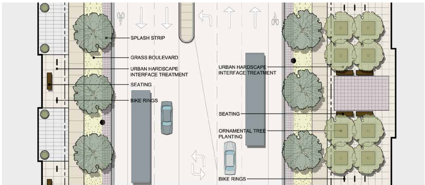
Figure 6.4.2c – Section M1-M1: Conceptual treatment along McLaughlin Road (towards Spine Road intersection) (35.0m ROW) with 4 thru lanes, left turn lane, island median, on-street bike lanes and street trees in grass boulevard adjacent to street-accessed commercial and Community Park/Recreation Centre/Village Square (looking north).
