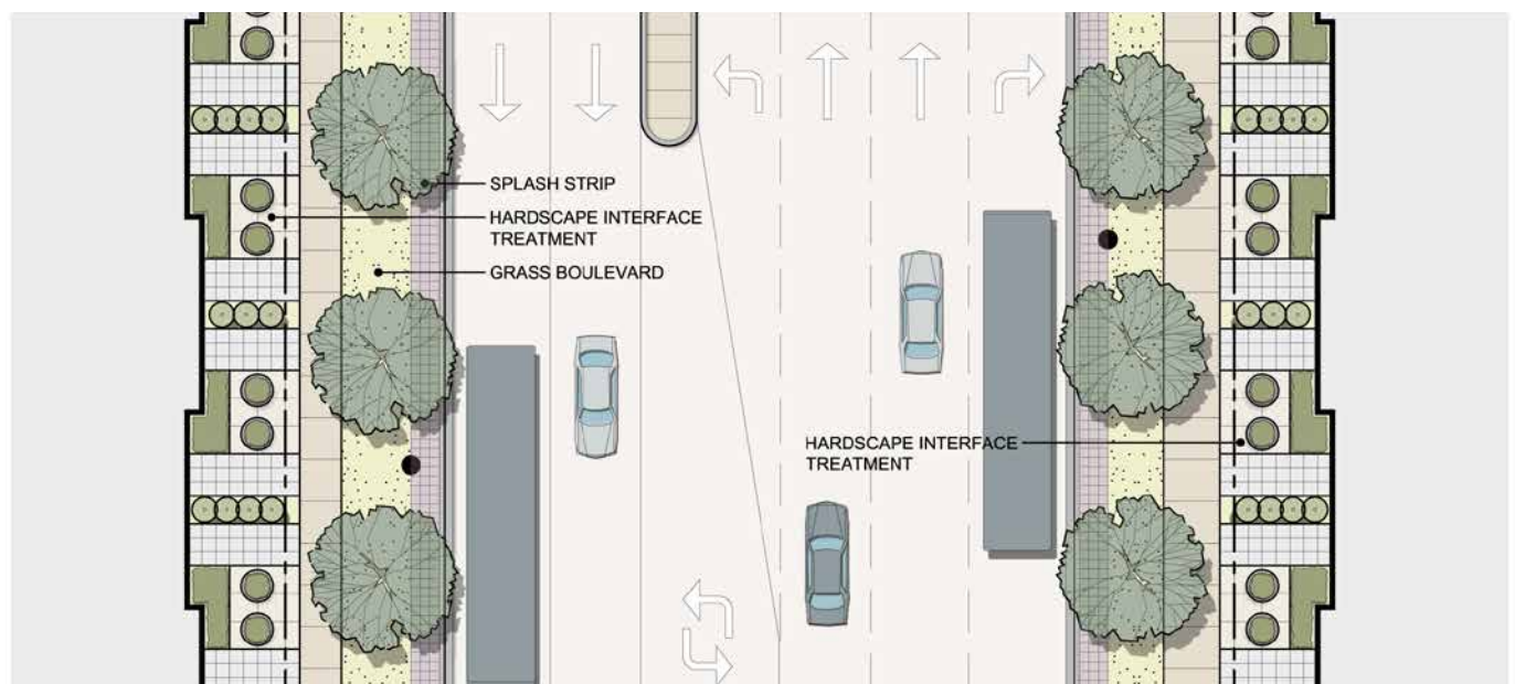
Figure 6.4.4a – Section D1-D1: Option 1 - Conceptual Spine Road treatment east of Collector Road F (34.0m ROW) with 4 thru lanes, left turn lane, island median at intersection and street trees in grass boulevard option (looking west).
