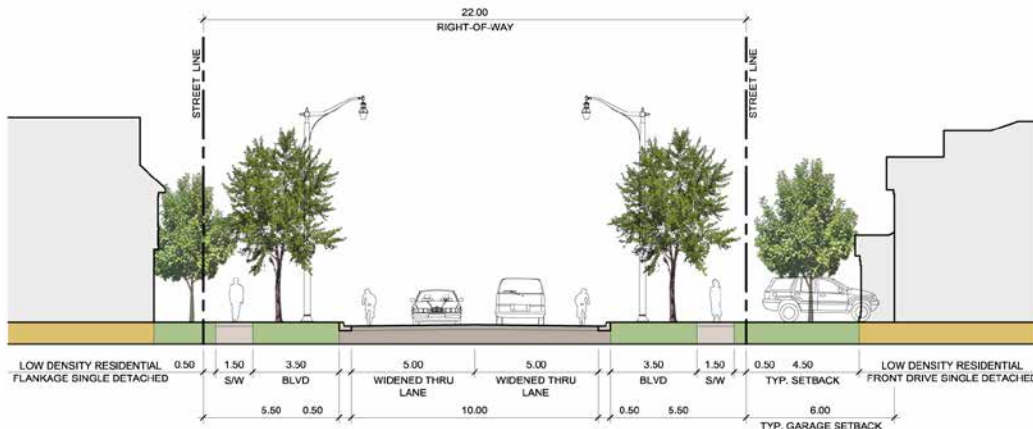
Figure 6.6b – Conceptual typical treatment for Collector Roads A, B, C, D, E, F and G (22.0m ROW) with 2 widened thru lanes to accommodate cyclists and street trees in grass boulevard.
