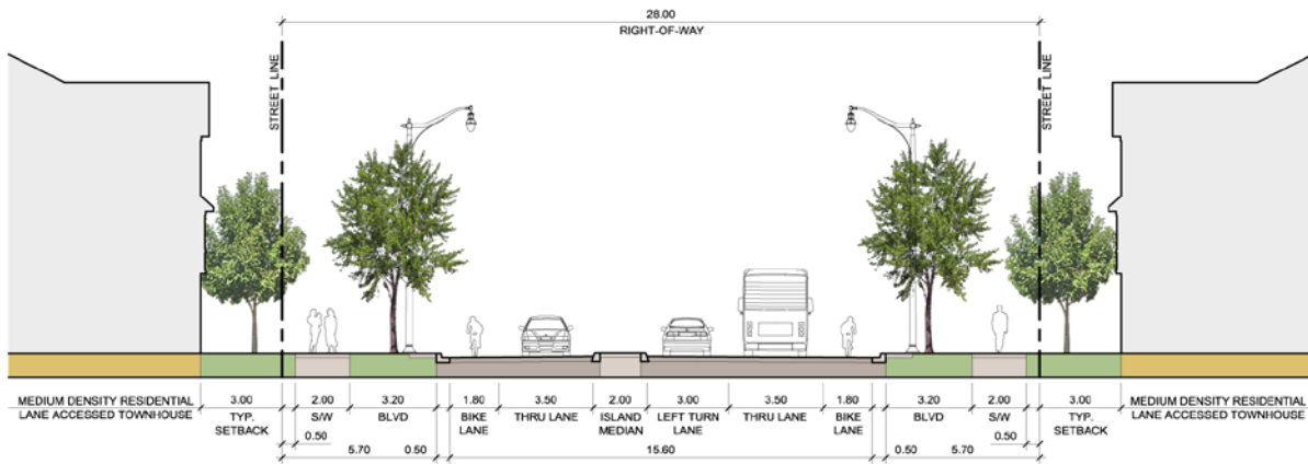
Figure 6.5b – Conceptual treatment along McLaughlin Road at the intersection with Collector Road A (28.0m ROW) with 2 thru lanes, left turn lane, island median, on street bike lanes and street trees in grass boulevard (looking north).
