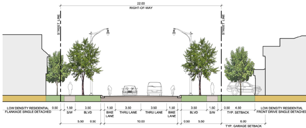
Figure 6.6a – Conceptual typical treatment for Collector Roads A, B, C, D, E, F and G (22.0m ROW) with 2 thru lanes, on-street bike lanes, no on-street parking and street trees in grass boulevard.
