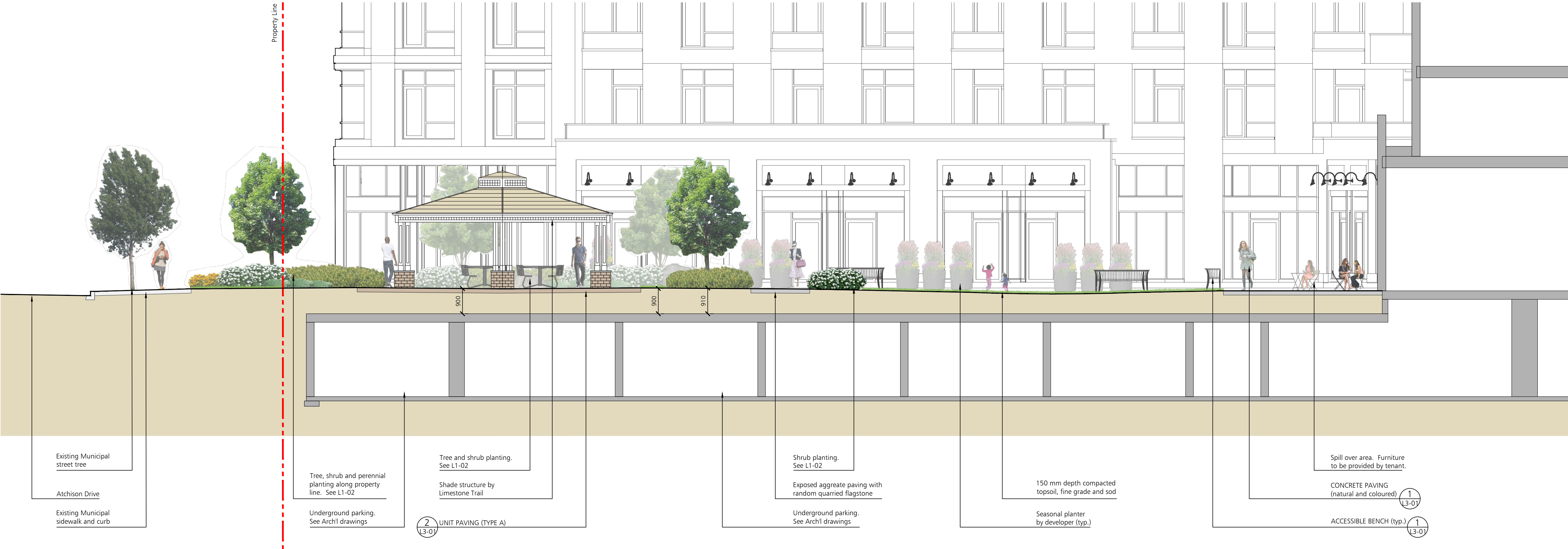
Section B - B' 1:750
