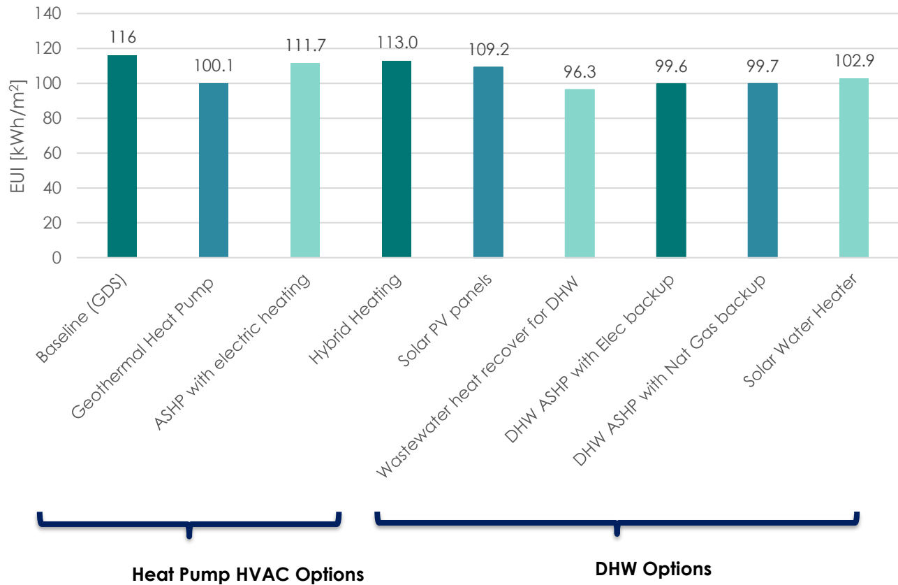
Figure 10 - Energy Use Intensity Results for Each HVAC System Assessed
