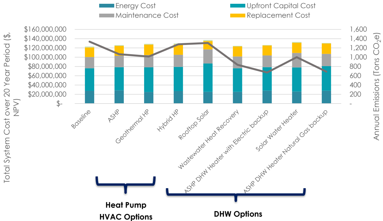
Figure 12: Total System Cost over 20 Year Period (NPV) of Each System Assessed Along with Annual CO 2 e Associated with Each Measure
