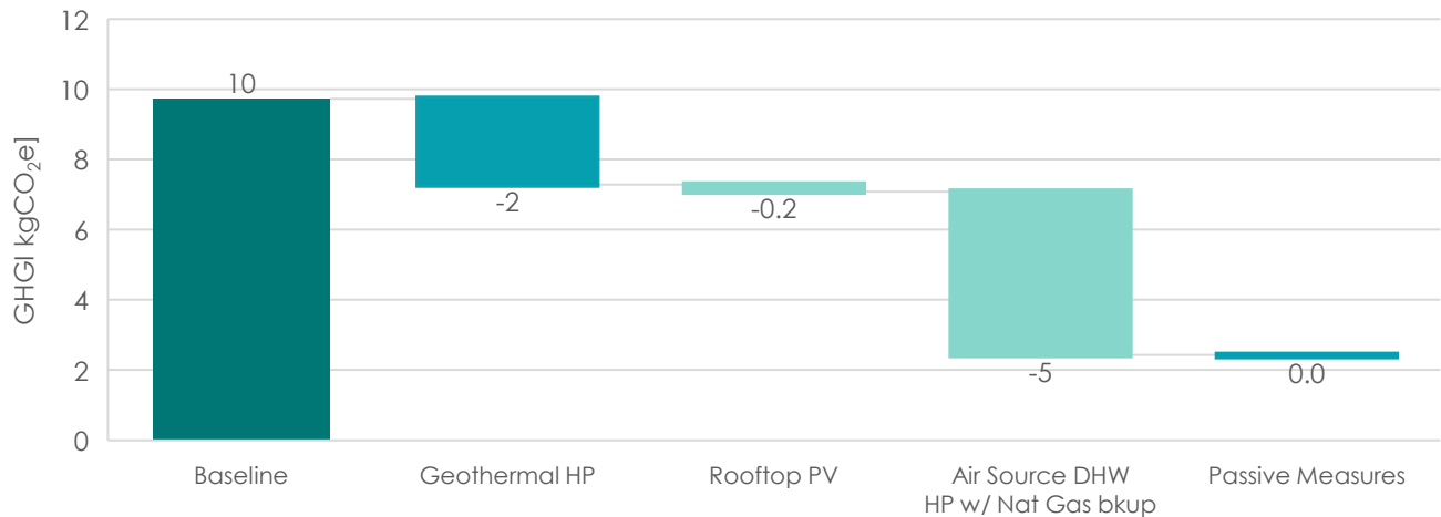
Figure 4: Greenhouse Gas Intensity Reduction Roadmap demonstrating GHGI reduction potential
