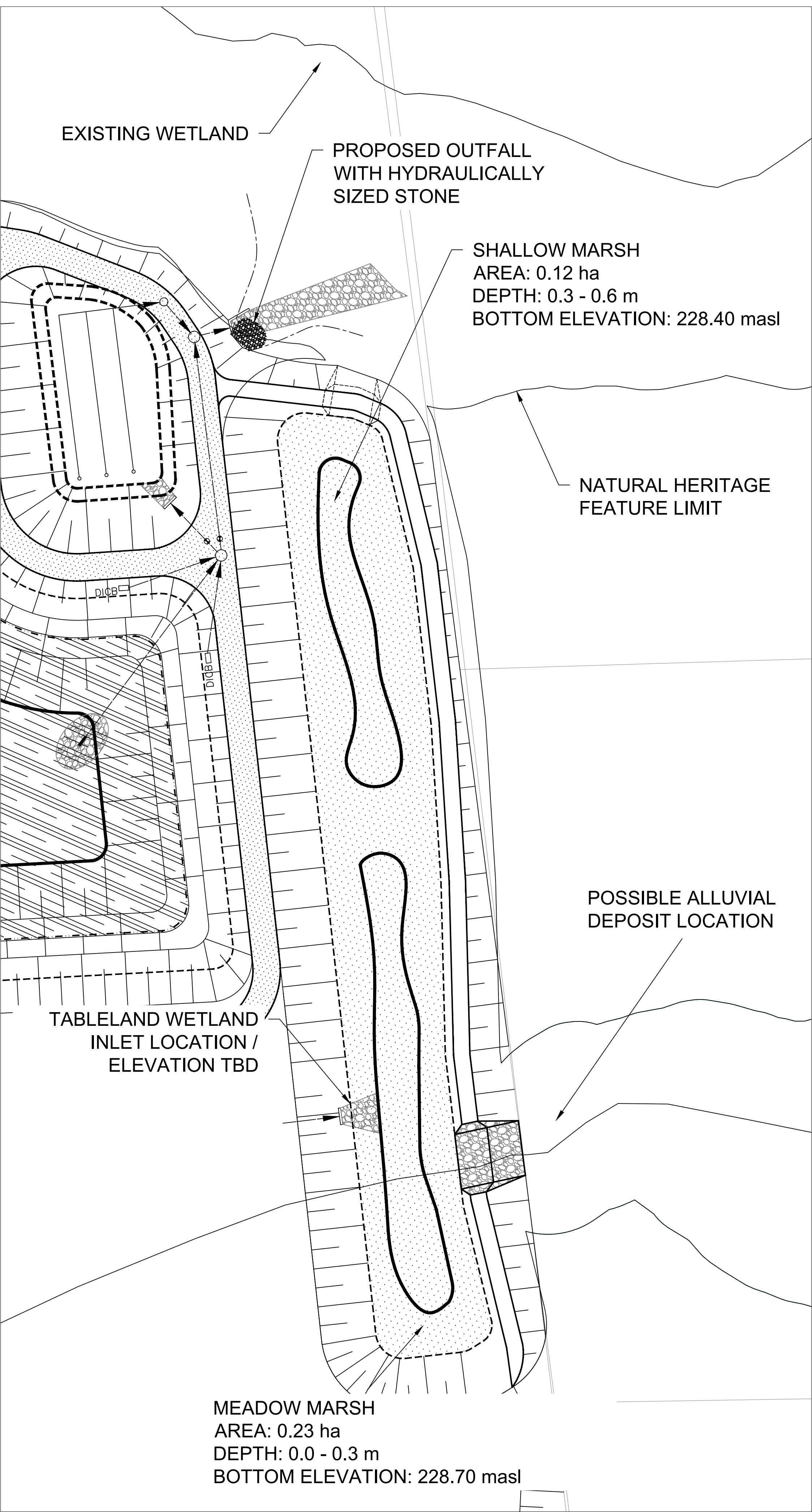
COMPENSATION WETLAND AREA 2 SCALE 1:500
