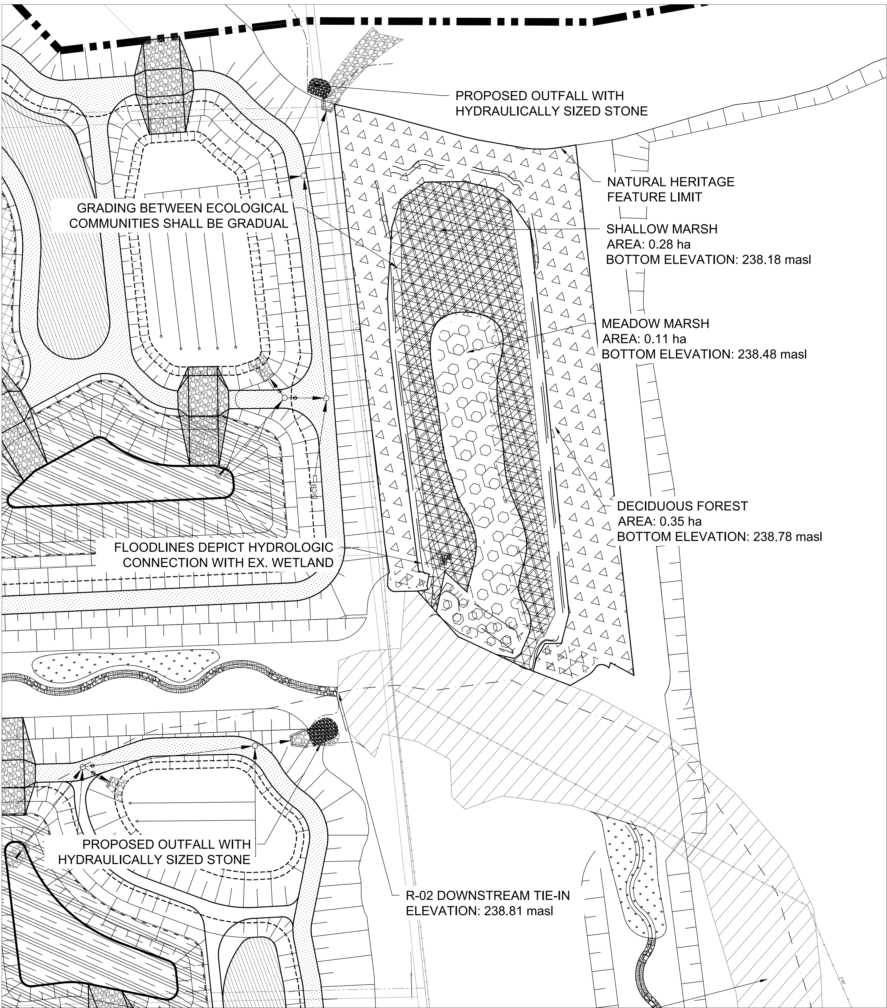
RELOCATION WETLAND AREA A SCALE 1:500
