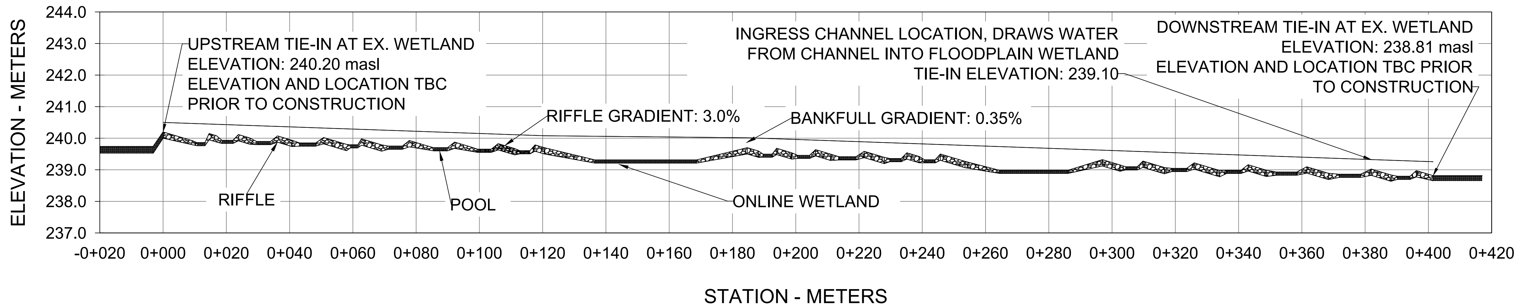
REACH 2 - PROPOSED PROFILE SCALE 1:750
