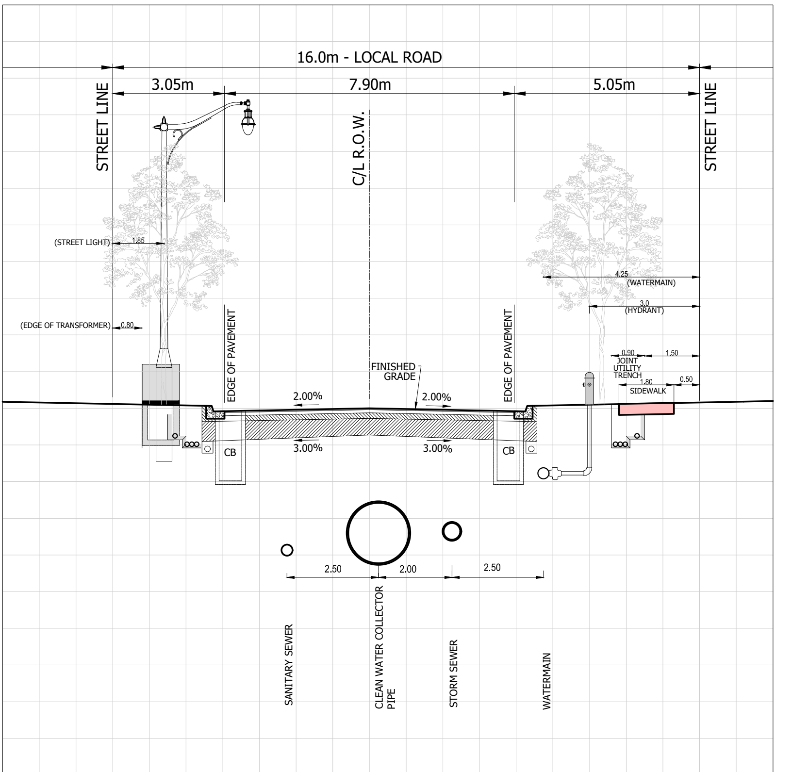
16.0m ROW CROSS SECTION WITH CWC (TYPICAL DETAIL)
