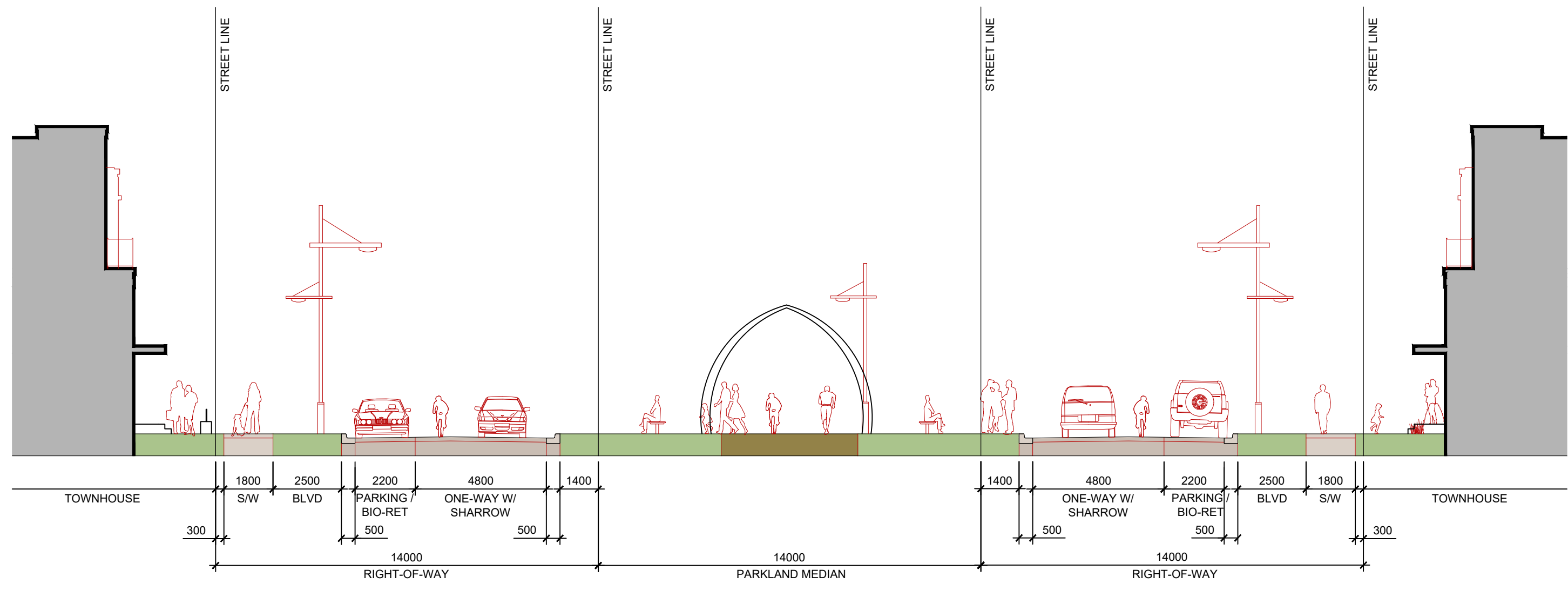
CENTRAL PROMENADE GREEN LINK STREET (ONE WAY - 14.0m R.O.W.) - OPTION A
