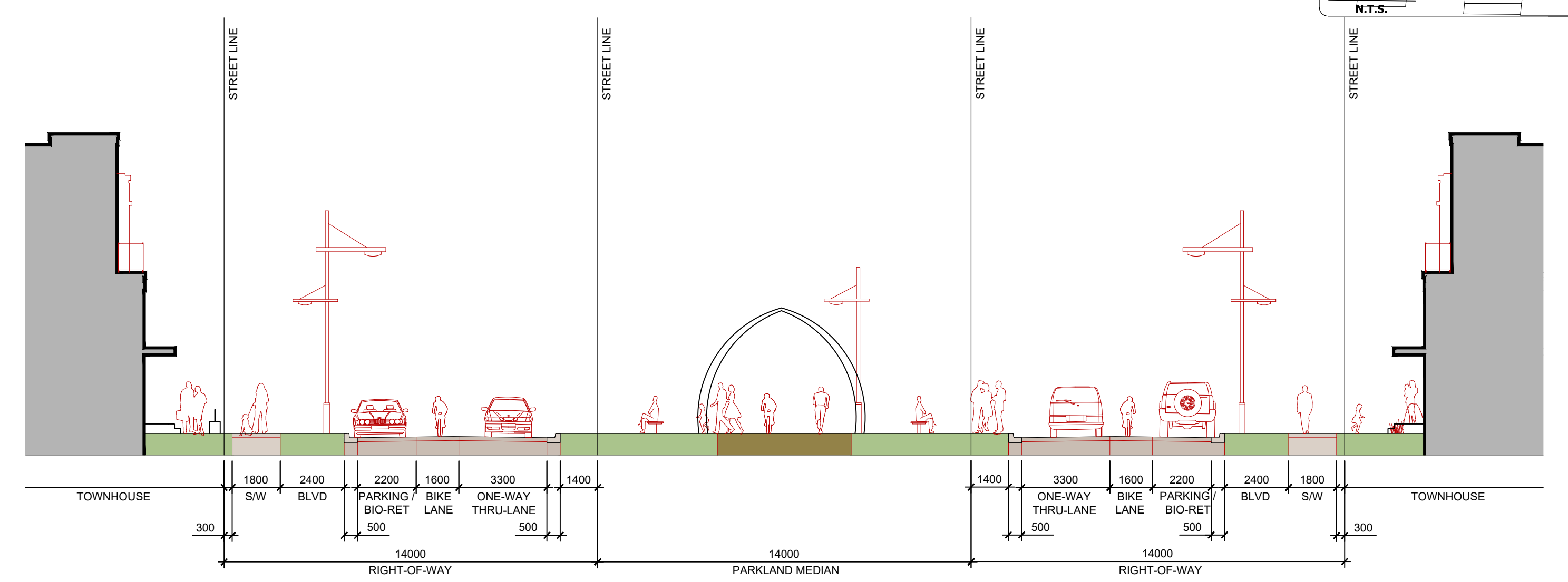
CENTRAL PROMENADE GREEN LINK STREET (ONE WAY - 14.0m R.O.W.) - OPTION B
