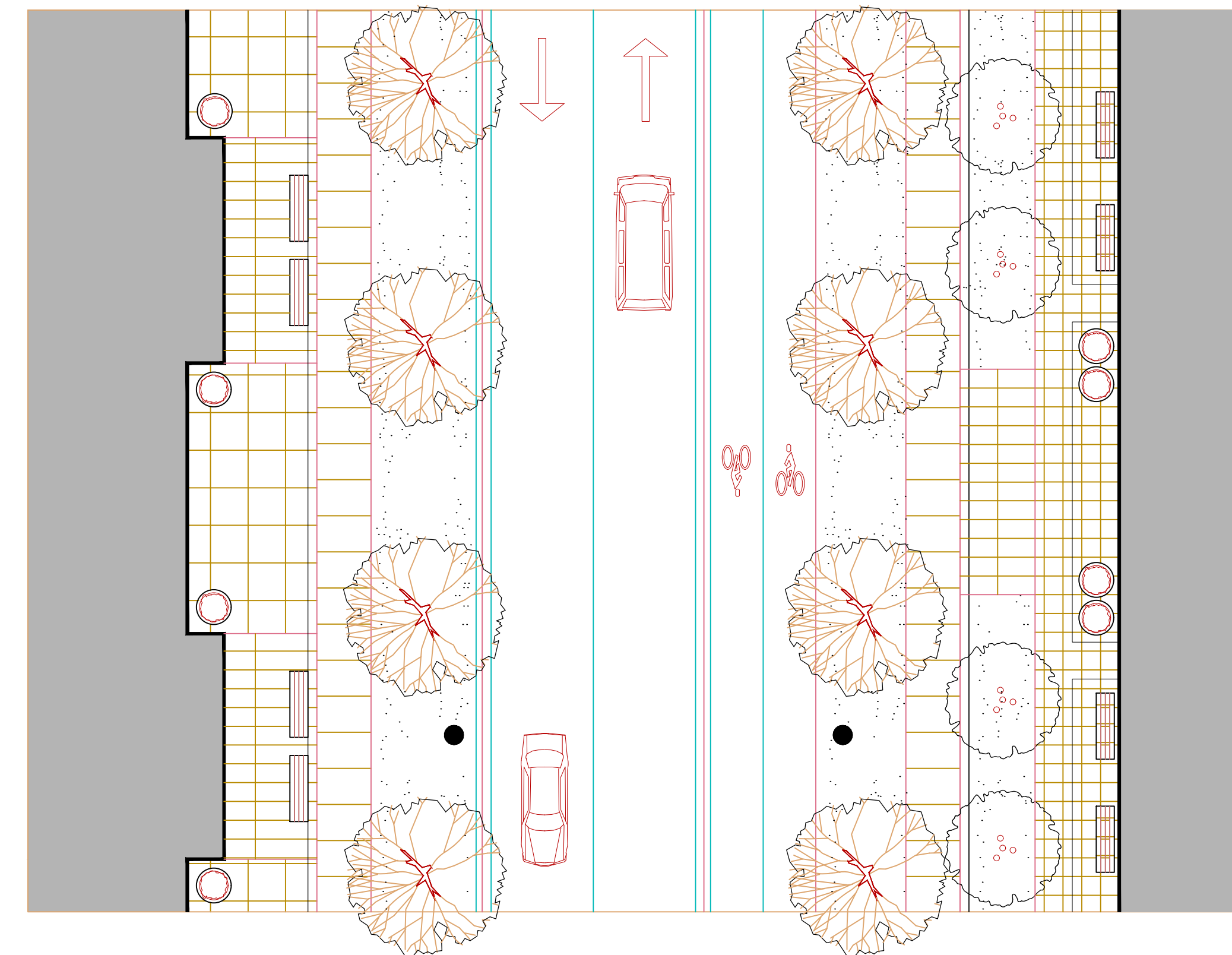
MAJOR COLLECTOR (EAST-WEST LINK) - 22.0m R.O.W. (OPTION 1)
