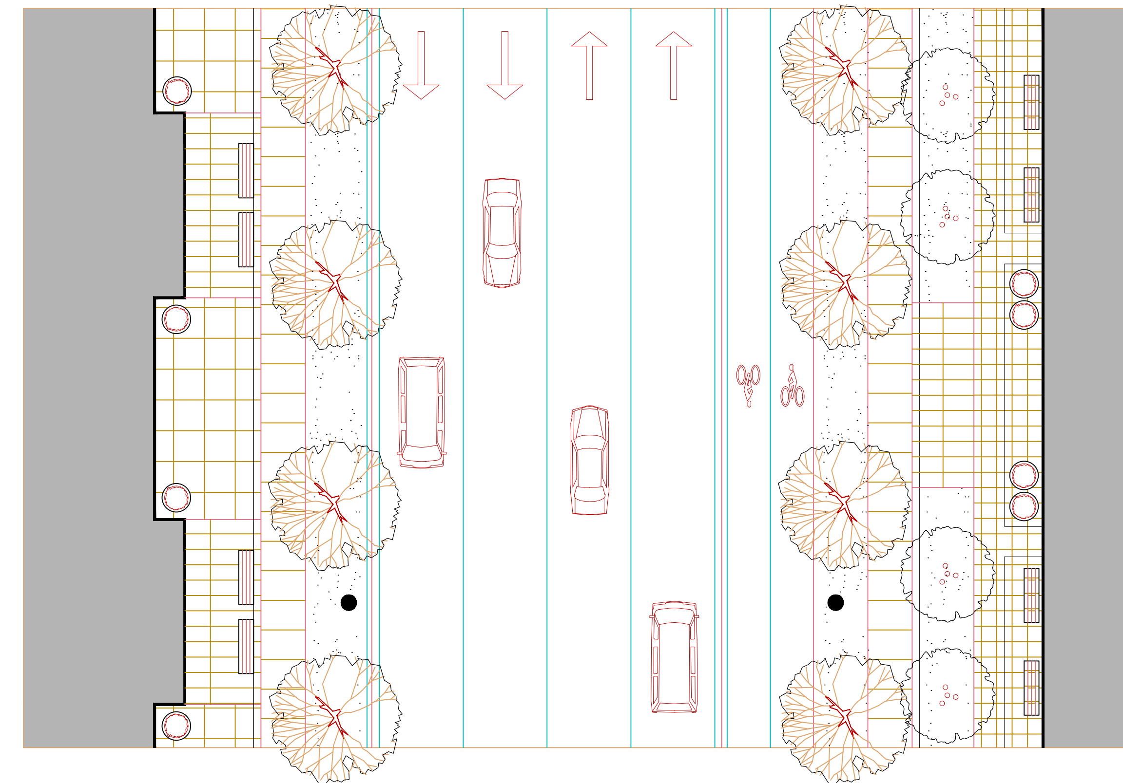
MAJOR COLLECTOR (EAST-WEST LINK) - 27.0m R.O.W. (OPTION 2)
