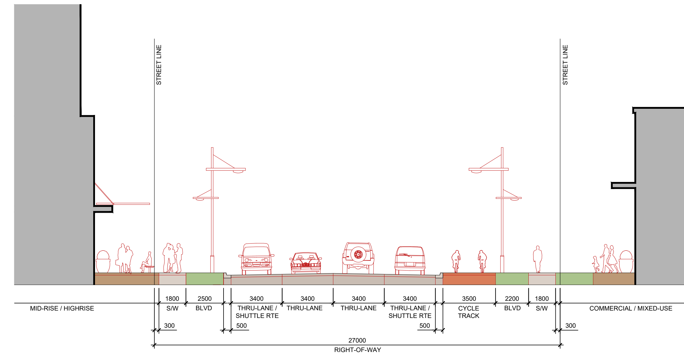
MAJOR COLLECTOR (EAST-WEST LINK) - 27.0m R.O.W. (OPTION 2)
