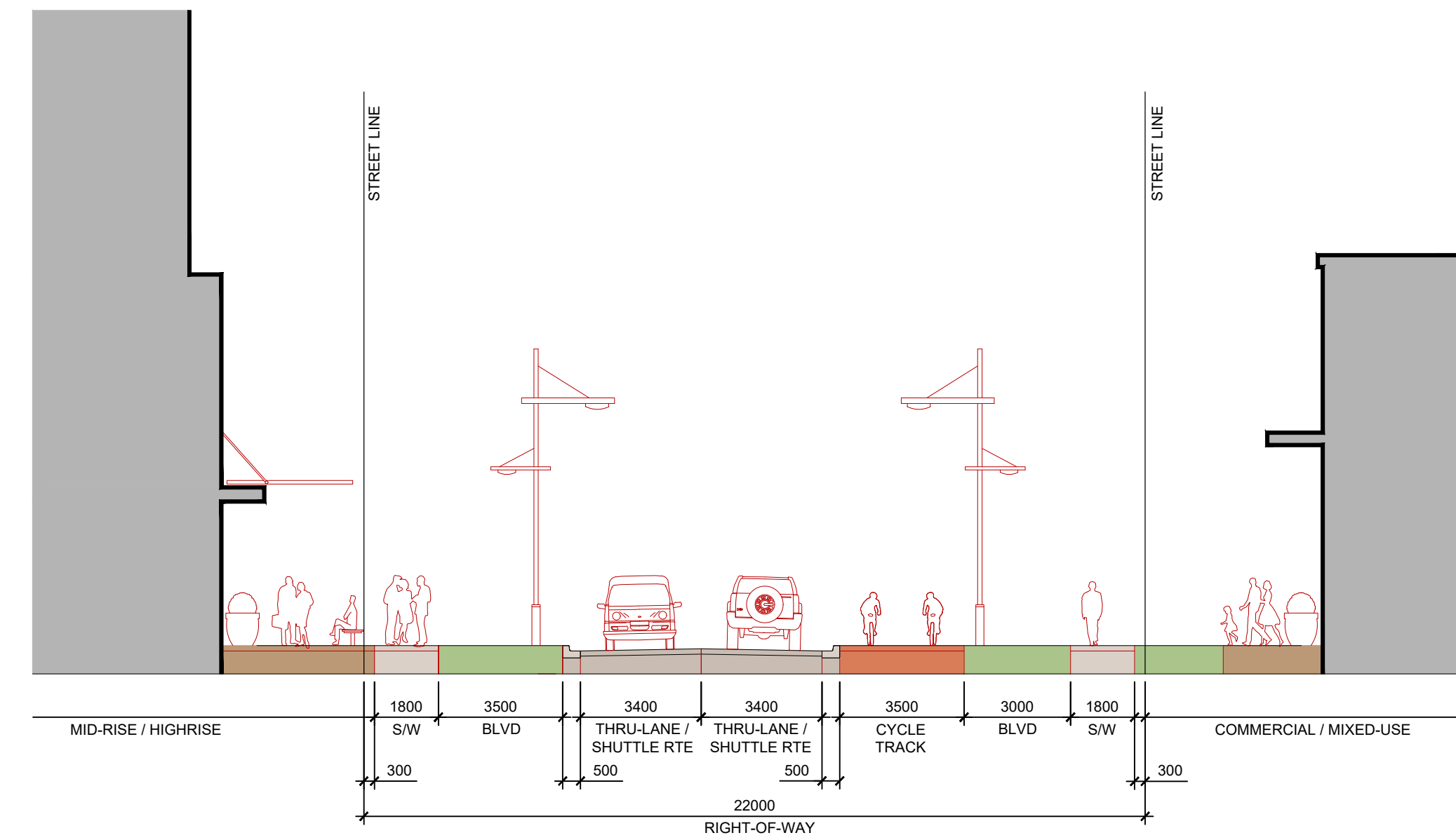
MAJOR COLLECTOR (EAST-WEST LINK) - 22.0m R.O.W. (OPTION 1)
