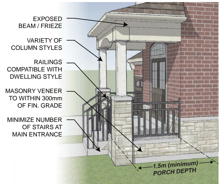
Figure 4.2.2: Typical porch design detail
