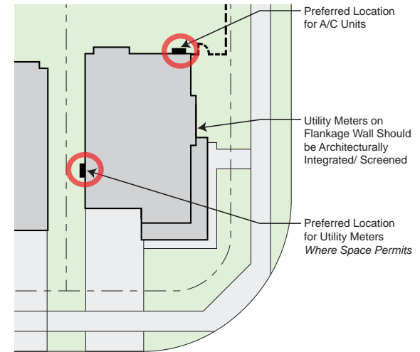
Figure 5.4.10a: Preferred location for utility meters for detached dwellings
