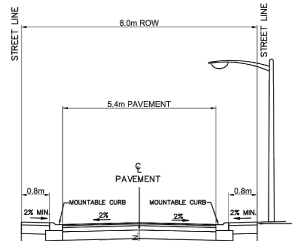
Figure 2.2g: 8.0m laneway
