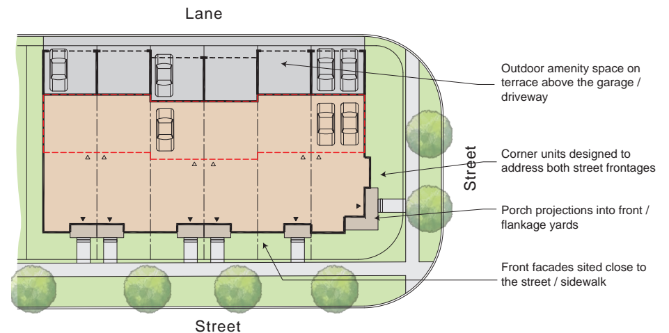
Figure 3.3.4.5: Conceptual plan layout for rear lane townhouses
