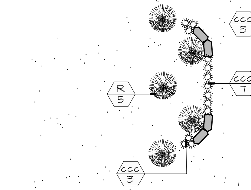
TYPICAL PLANTING LAYOUT TYPICAL DETAIL
