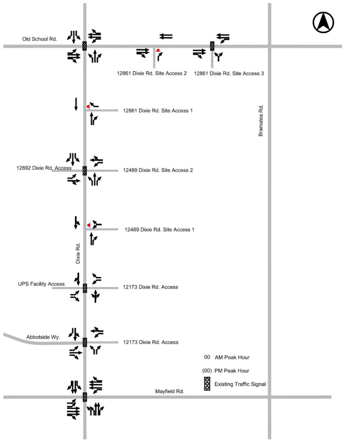
FIGURE 4 FUTURE LANE CONFIGURATION AND TRAFFIC CONTROL
