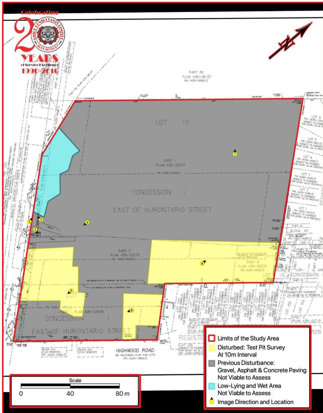
MAP 6 DETAILED PLAN OF THE STUDY AREA (AFTER DAVID B. SEARLES SURVEYING LTD. 2021)
