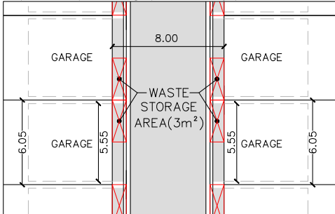
DETAIL 'B' - LANEWAY WASTE STORAGE
