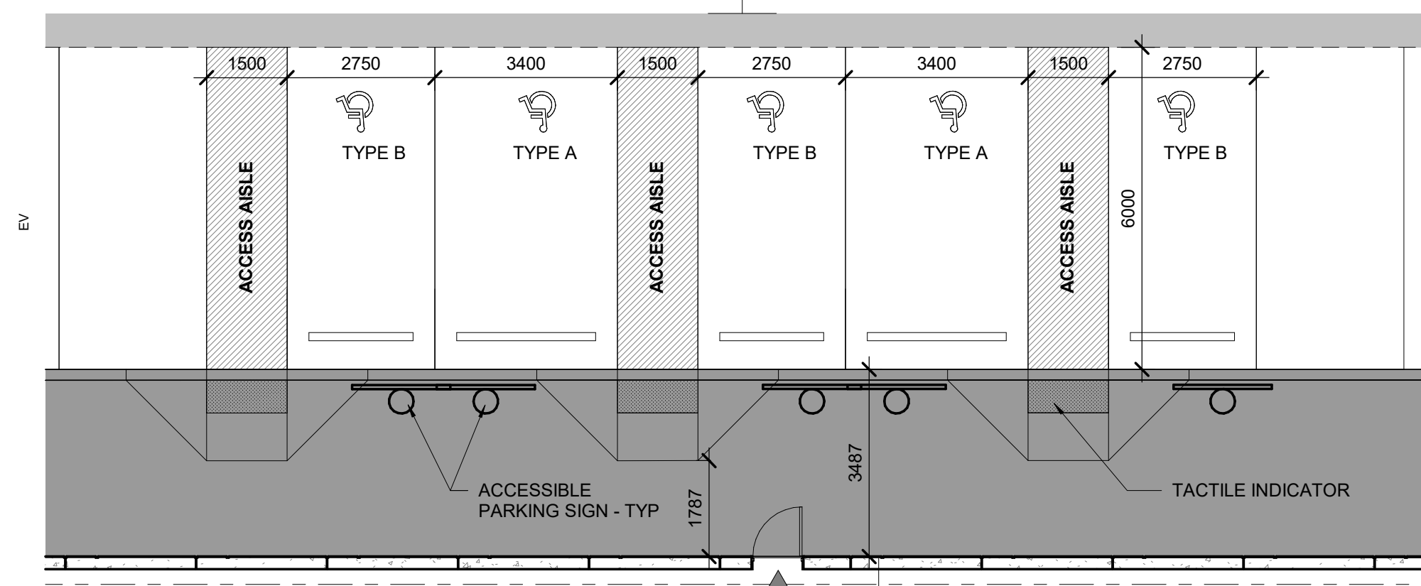
D3 ENLARGED SITE PLAN - ACCESSIBLE PARKING SCALE: 1 : 100
