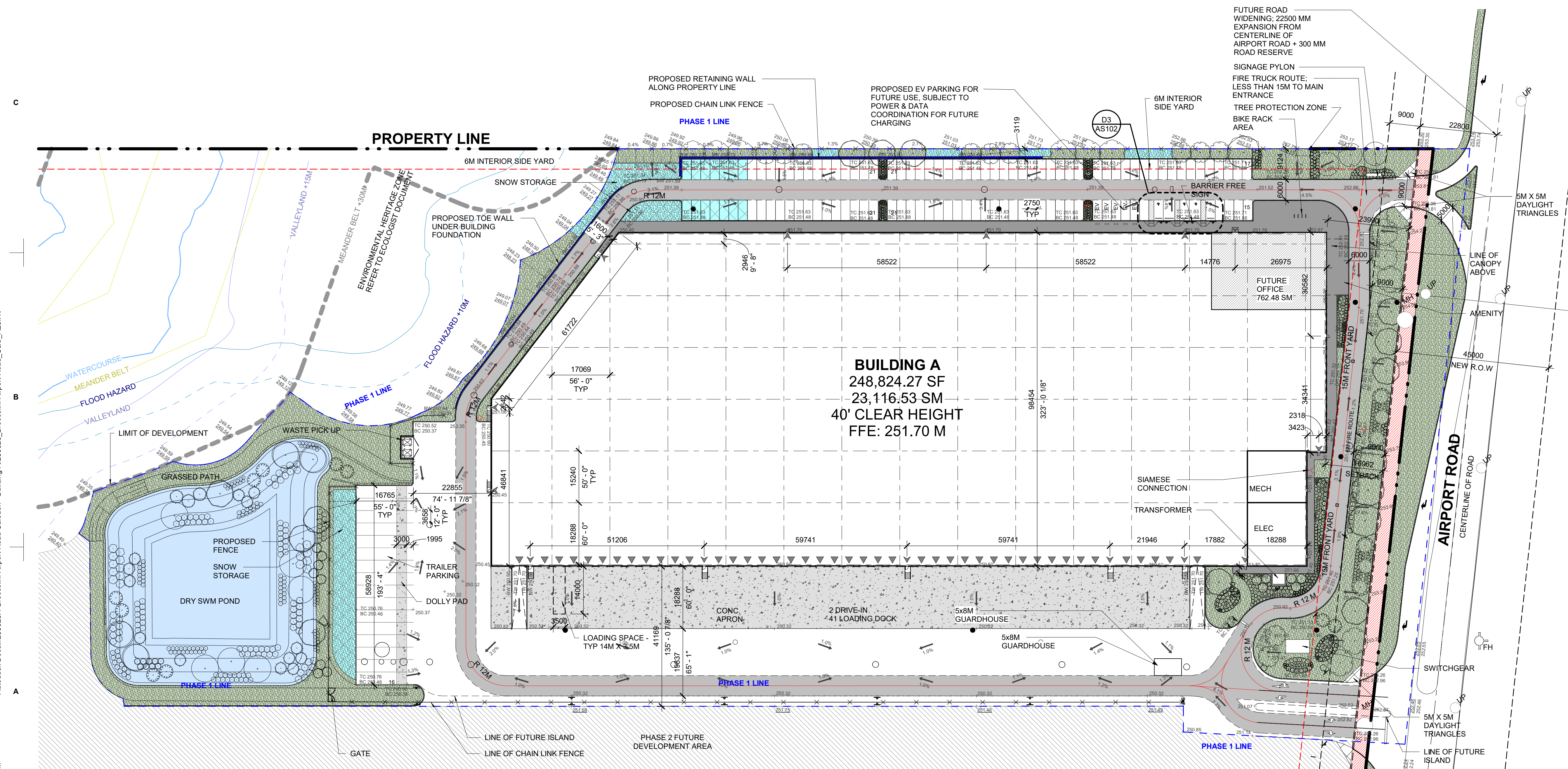
OVERALL SITE PLAN - BUILDING A
