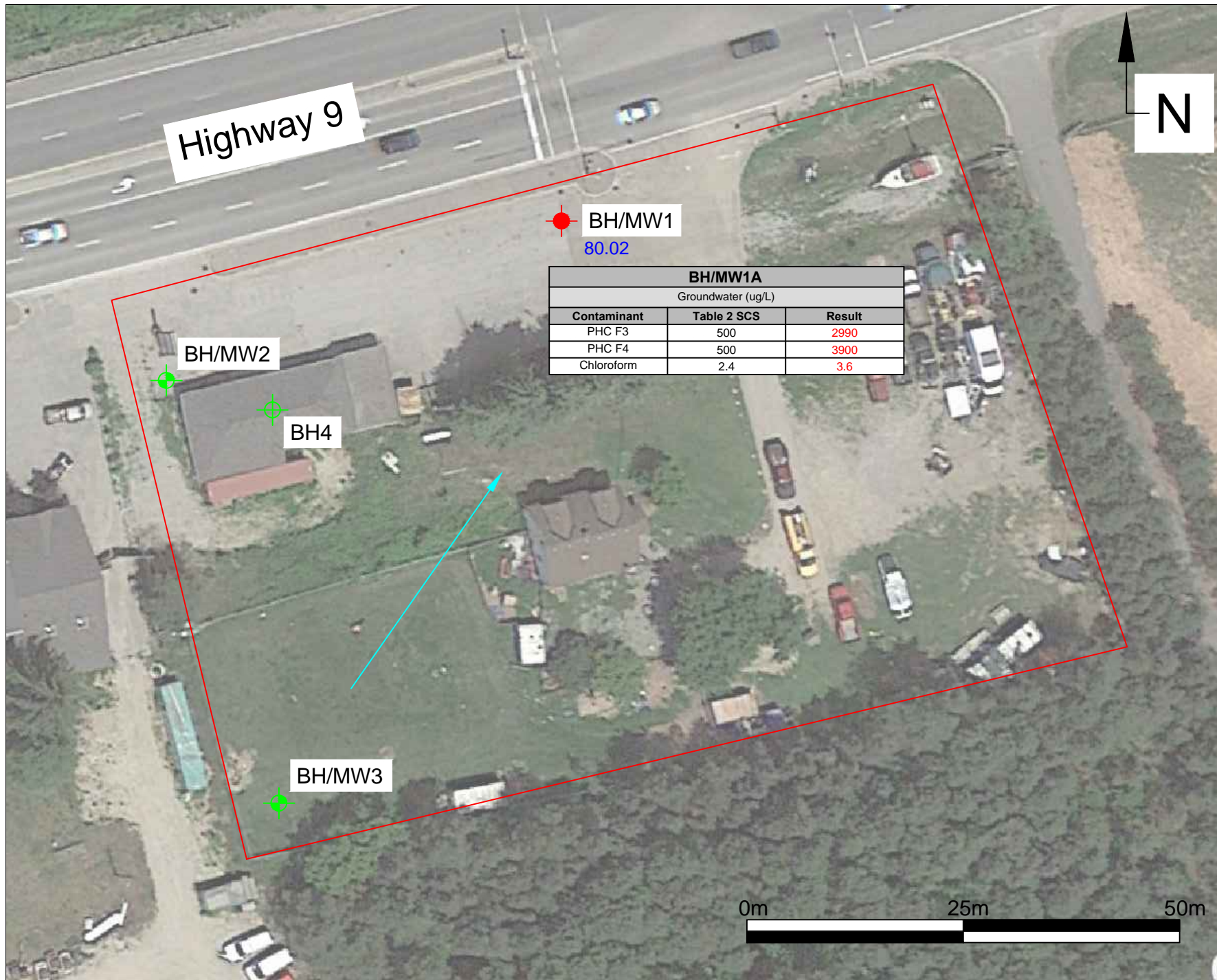
Title: Figure 2: Site Plan
